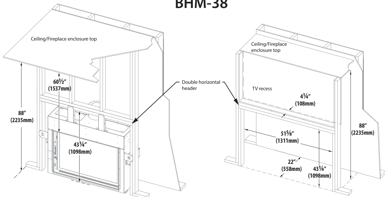
FIGURE 2.9 BHM-38 Unit Wall Enclosure Rough Opening
