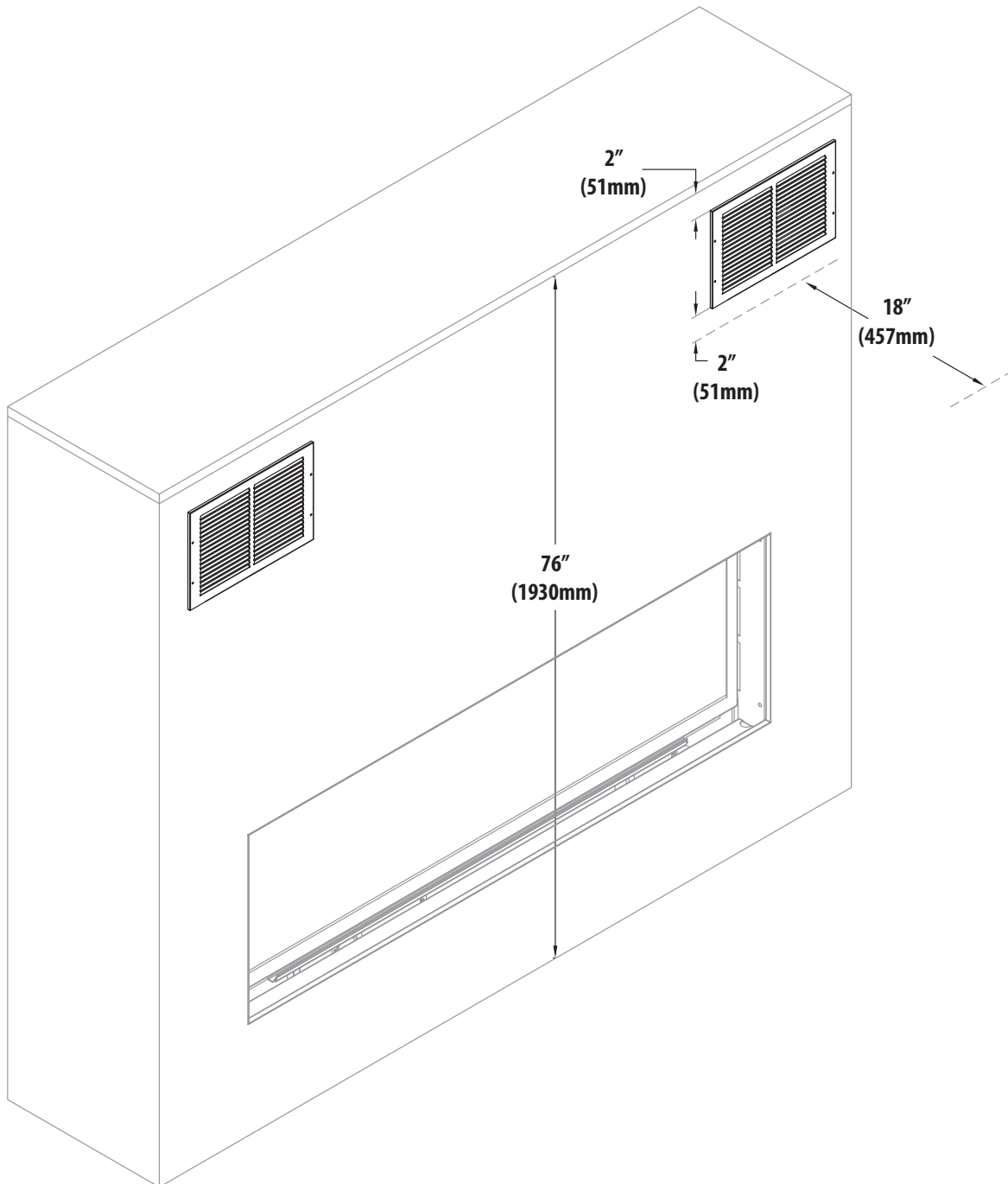
FIGURE 2.13 CLW-ST Front Facing Clearances
