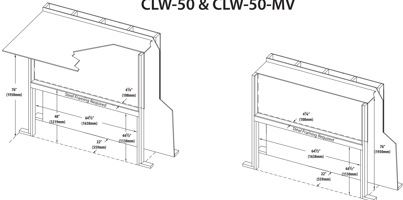
FIGURE 2.4 CLW-50 Unit Wall Enclosure Rough Opening
