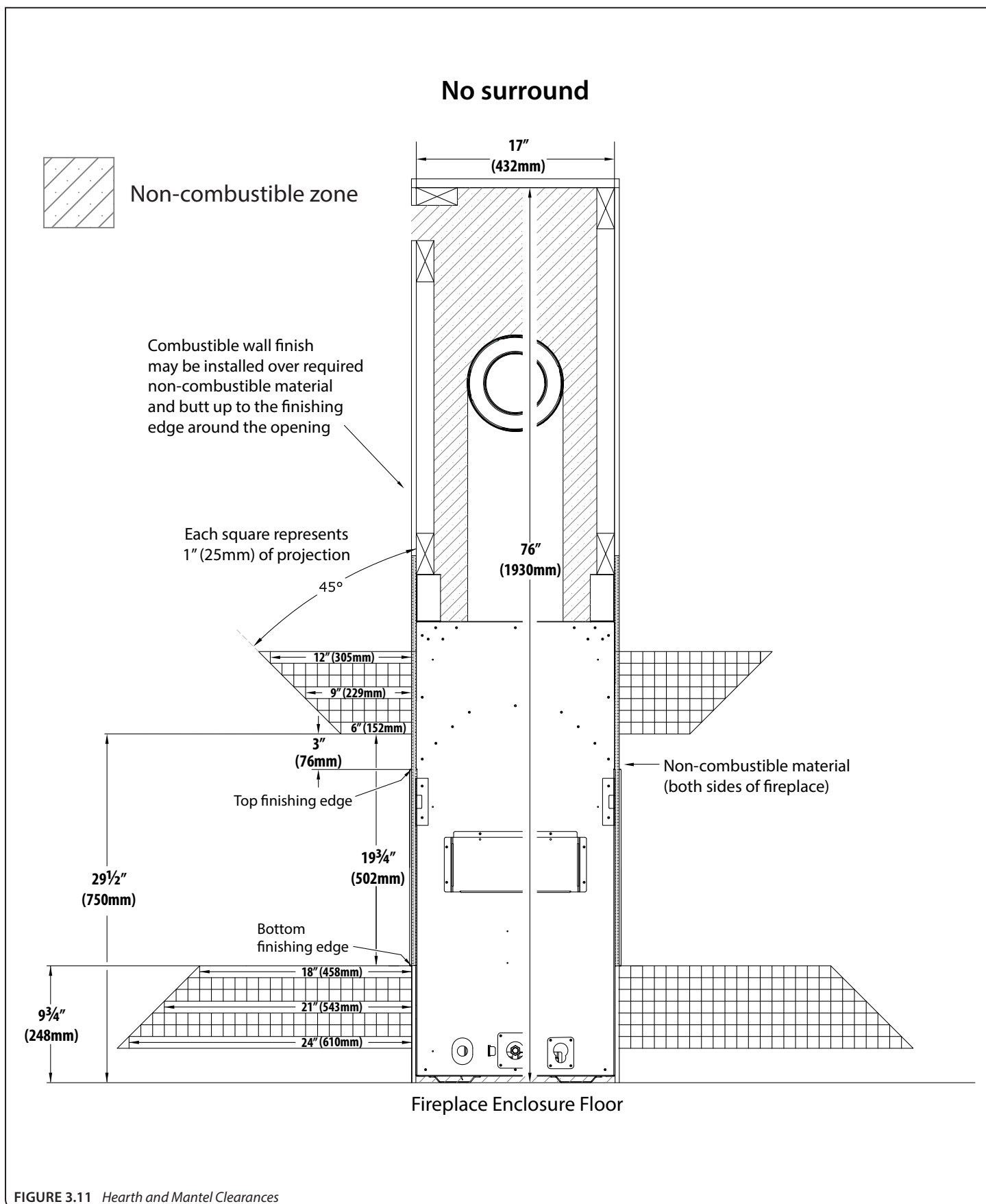
FIGURE 3.11 Hearth and Mantel Clearances
