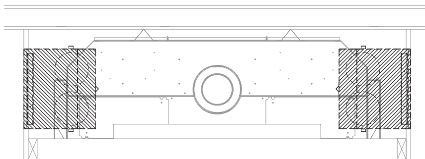
#KZK-1510A side wall outlet
