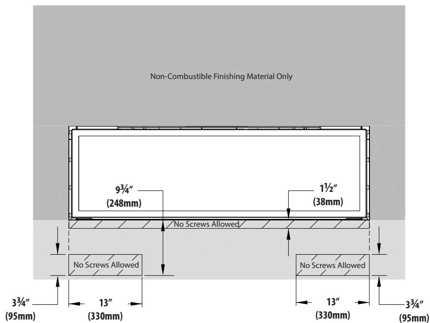
FIGURE 3.1 Minimum Non-combustible Finishing Dimensions
