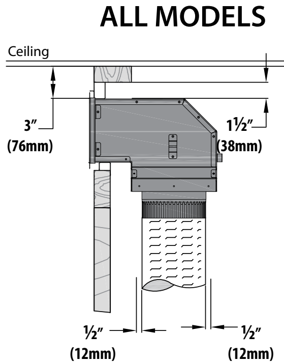
FIGURE 2.2 Minimum Clearances for Plenum Air Discharge to Ceiling
