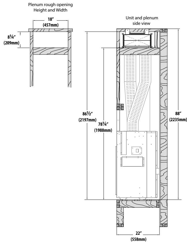
FIGURE 2.7 BHM-44 Rough Opening and Framing for #KZK-1510A
