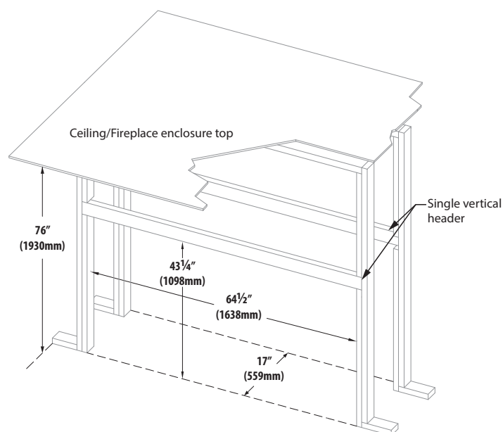
FIGURE 2.6 CLW-ST Unit Wall Enclosure Rough Opening
