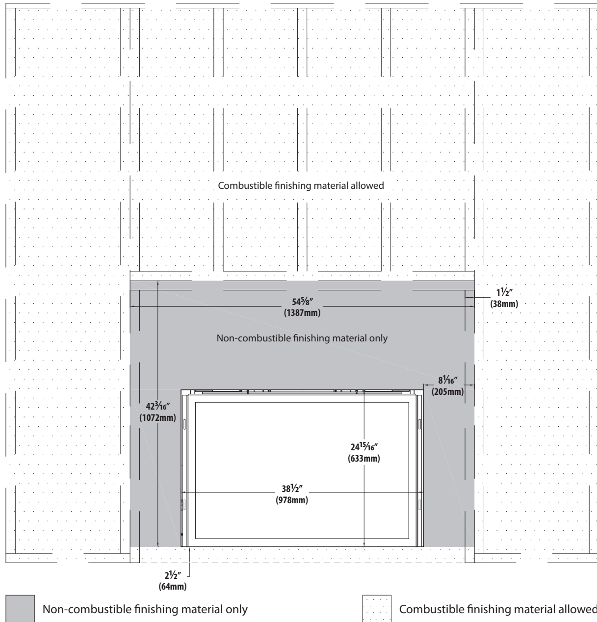
FIGURE 3.3 Minimum Non-combustible Finishing Dimensions
