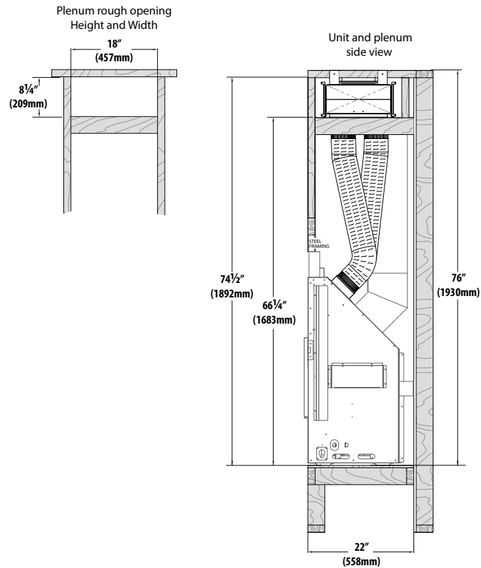
FIGURE 2.3 CLW-50 Rough Opening and Framing for #KZK-1510A
