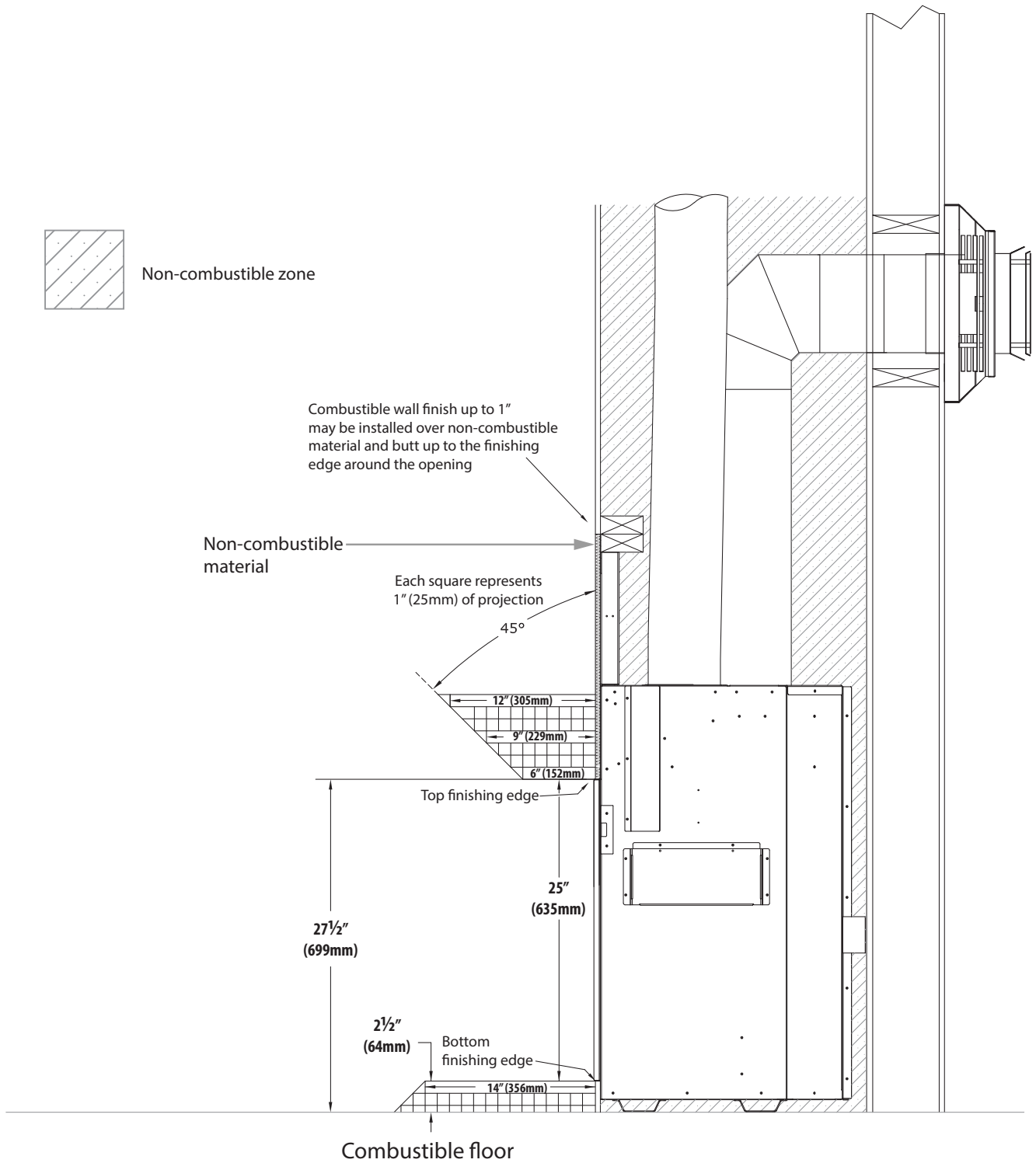
FIGURE 3.12 Hearth and Mantel Clearances
