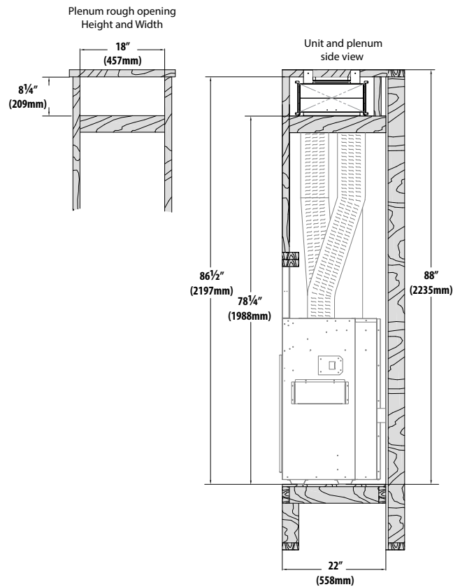
FIGURE 2.10 BHM-38 Rough Opening and Framing for #KZK-1510A
