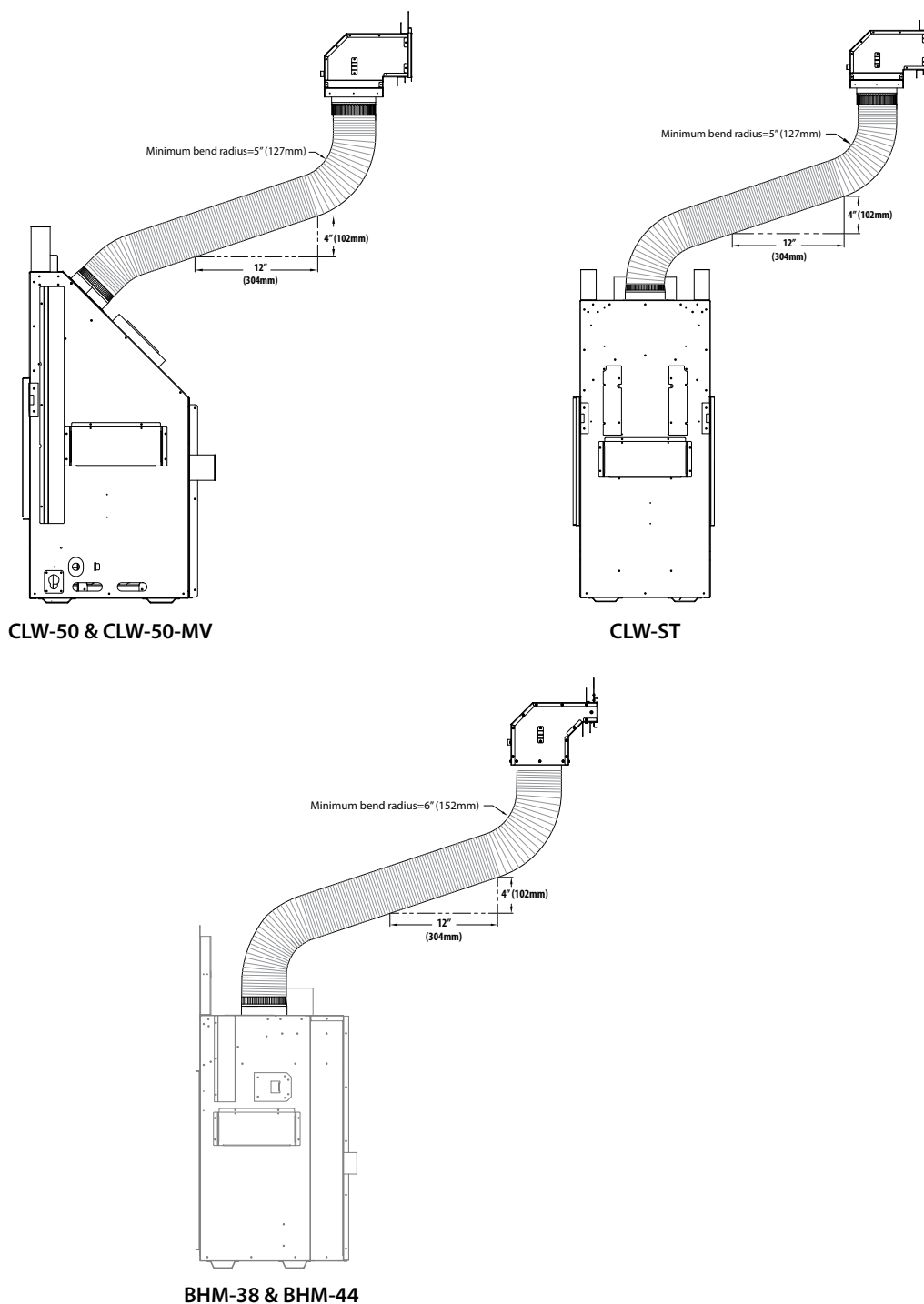
FIGURE 1.8 Minimum Vent Pipe Run - only (1) plenum shown
