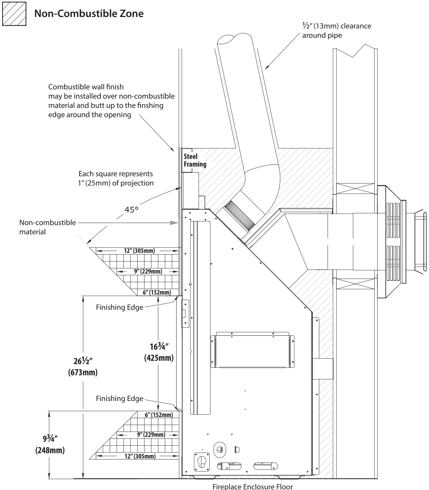
FIGURE 3.10 Hearth and Mantel Clearances
