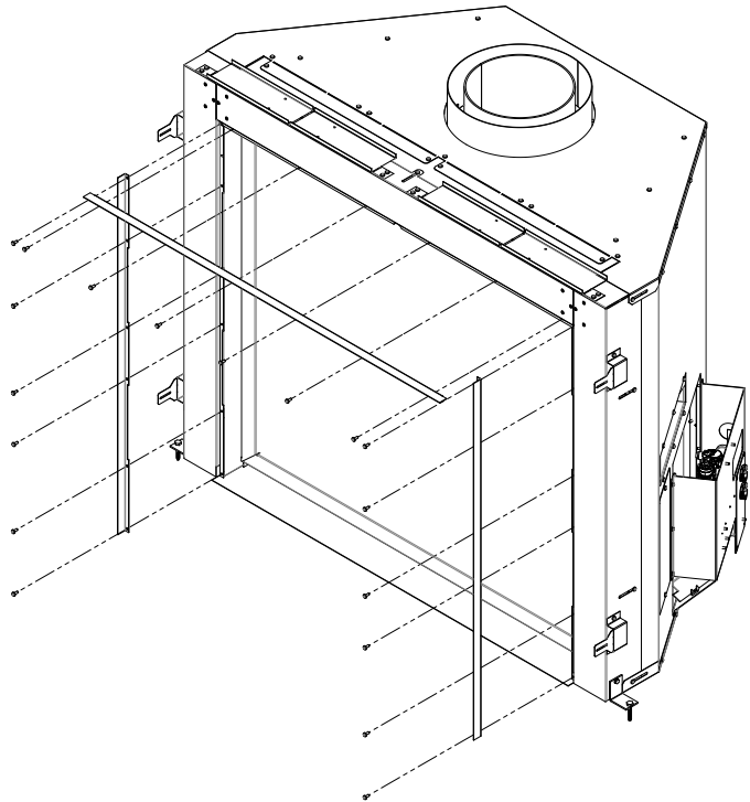
Figure 29: Finishing Edge Removal/Installation
