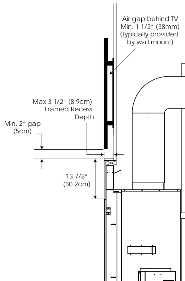
Figure 55: Recess Minimum TV Install
