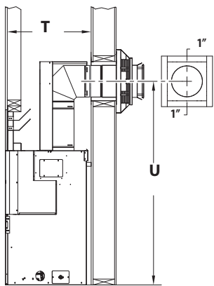
PROPANE MINIMUM HORIZONTAL TERMINATION
