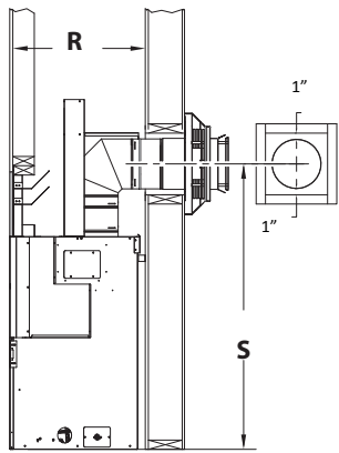
NATURAL GAS MINIMUM HORIZONTAL TERMINATION
