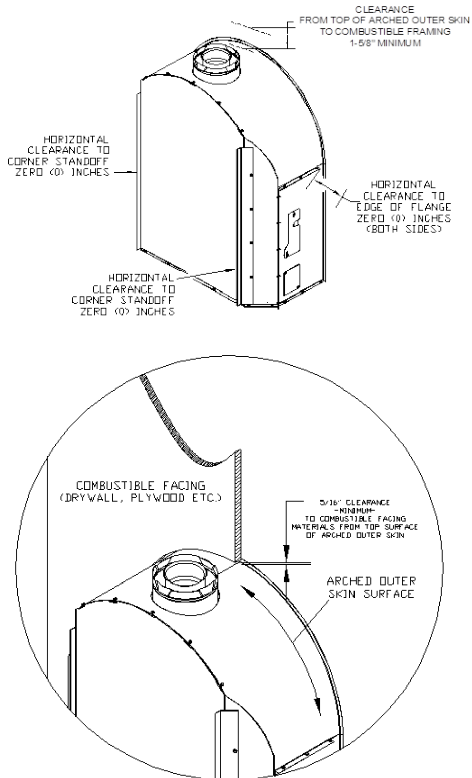
Figure 3-14 CLEARANCES TO APPLIANCE BODY
