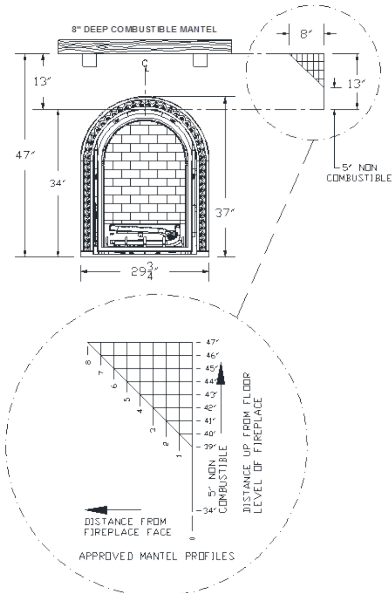
Figure 3-16 Mantel Clearances
